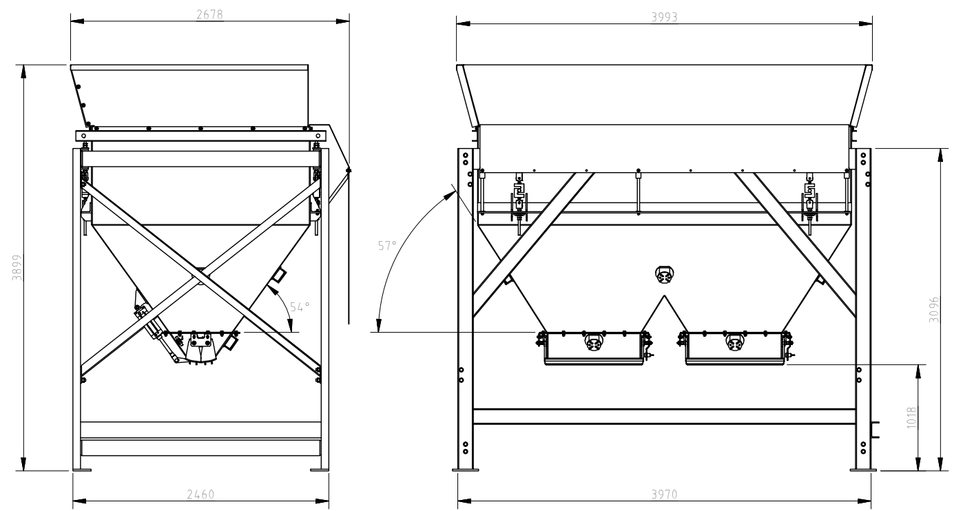
HORIZONTAL TYPE
