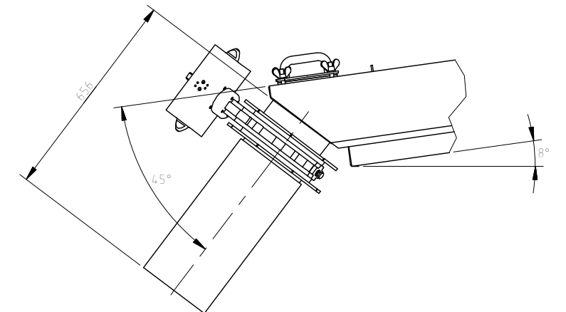
45 DEG DISCHARGE OPTION
