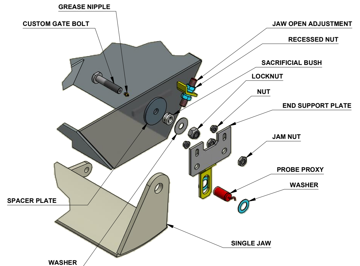
SINGLE JAW GATE
