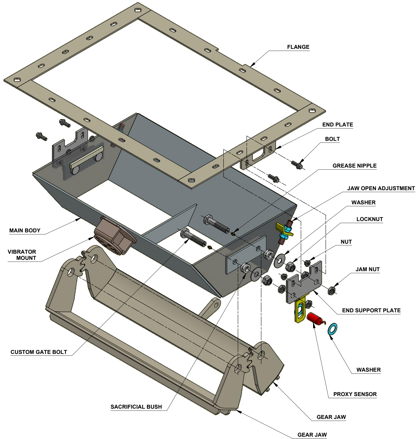
DOUBLE JAW GEAR GATE
